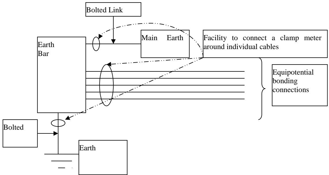
Figure 1. Earthing System
