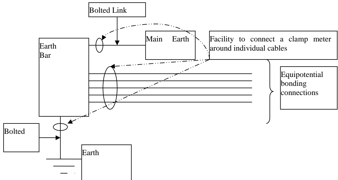
Figure 1. Earthing System
